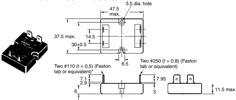
G3NE-205T(L)/210T(L)/220T(L)-(-2)(US)
